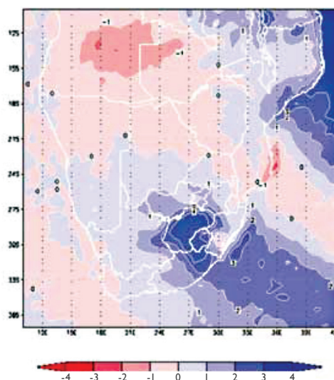
Figure 6: Projected change in the annual frequency of extreme rainfall events (>20mm day -1 ) by 2071–2100 compared to 1961–1990 over the southern African region (Davis, 2011).
