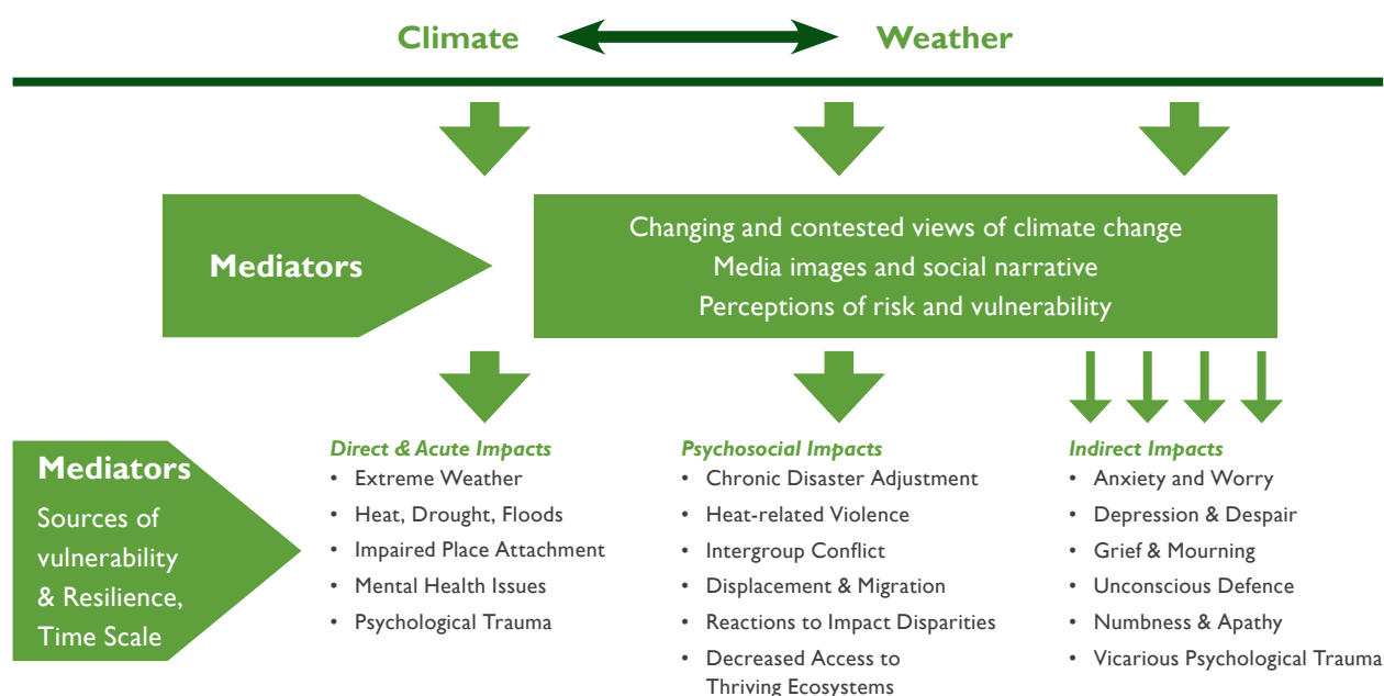
Figure 4: Climate change: differentiating between classes of psychological impacts (Doherty and Clayton, 2011).
