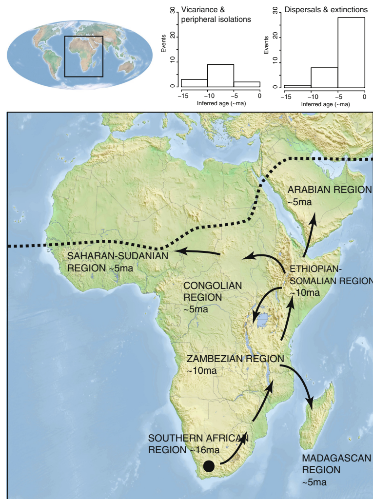
Figure 2 Biogeographic scenario for Aloe . Distribution and biogeographic scenario for Aloe inferred from nucleotide and plastid data for 228 taxa in Xanthorrhoeaceae subfamily Asphodeloideae. Enlarged map shows the natural distribution of Aloe , with northernmost limits indicated by dashed line. Direction and timing of diversification events inferred from ancestral state reconstruction and penalised likelihood dating are shown by arrows. Histograms show branch-based (dispersal and extinction) and node-based (vicariance and peripheral isolations) events in speciation processes since the divergence of the Aloe crown group ~16 Ma.
